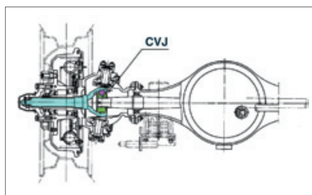
Drive Axle
